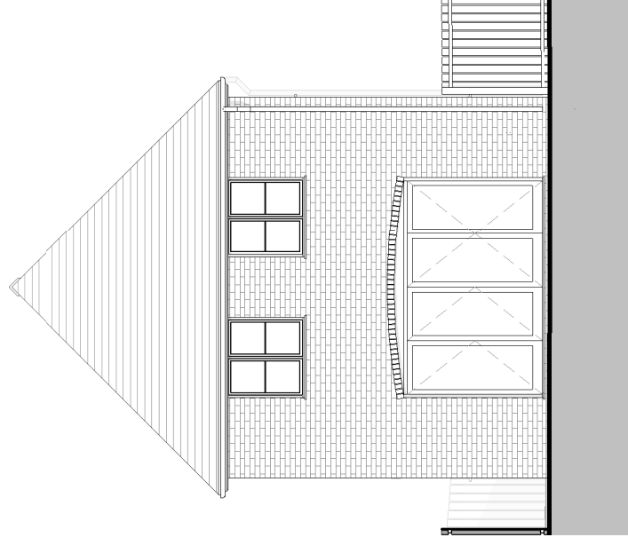
House 3 - East Elevation as Proposed 1 : 100
