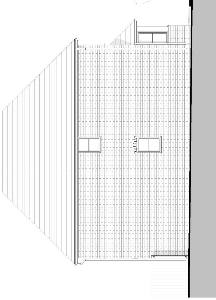
House 3 - North Elevation as Proposed 1 : 100
