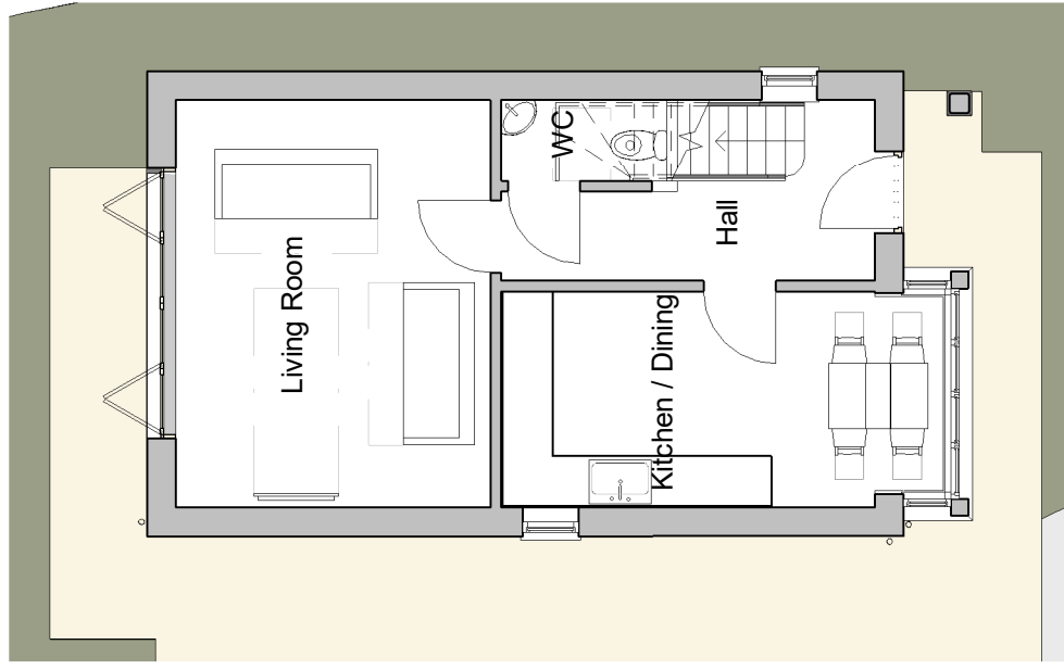
House 3 - Ground Floor Plan as Proposed 1 : 100
